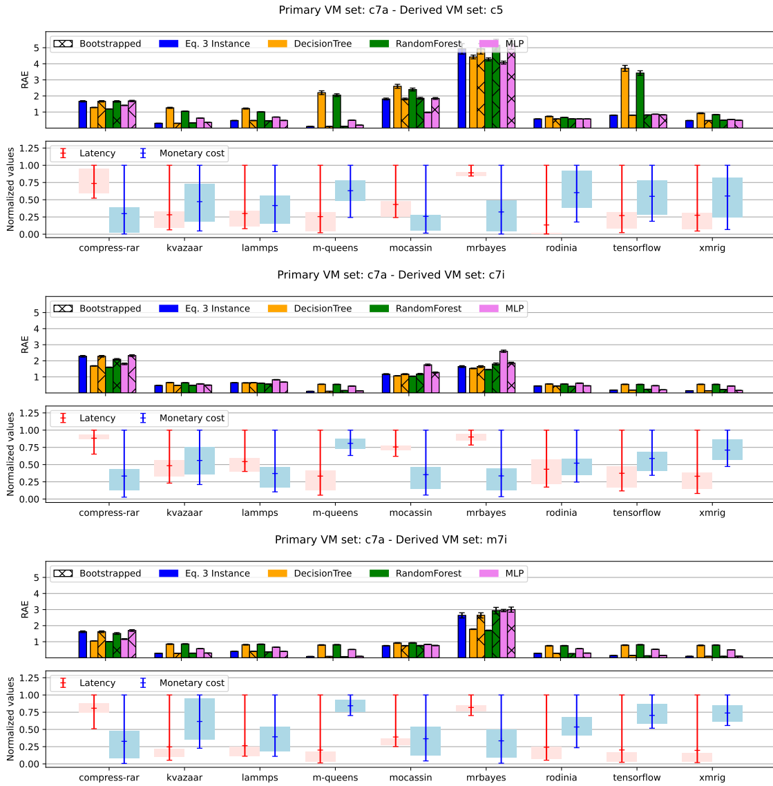
Fig. 6. Results for C5, C7i and M7i families for all benchmark applications, using C7a family as a primary VM set, three samples ( k = 3 ) for the primary VM set and one sample for each.
